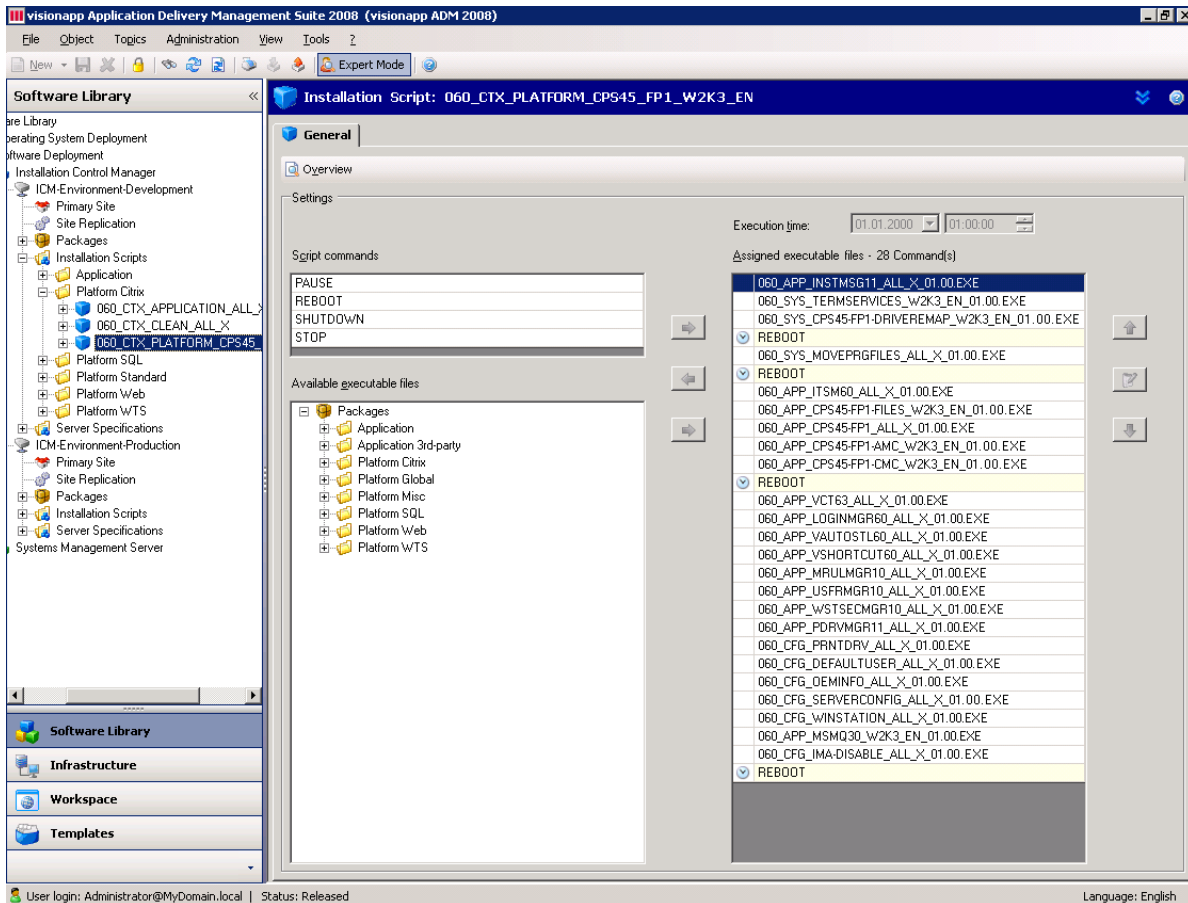
visionapp Server Management status basic configuration of the installation environment
